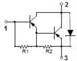
PIN 1. BASE 2. COLLECTOR 3. EMITTER TO-220C package
