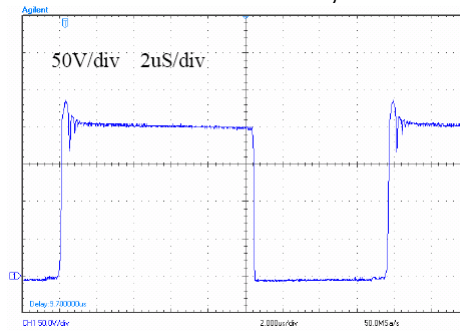
V in =110V, I o =1A
