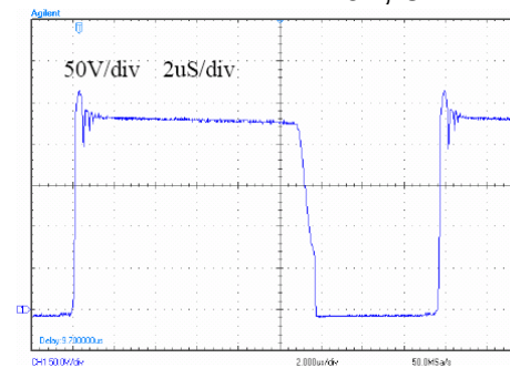
V in =220V, I o =1A
