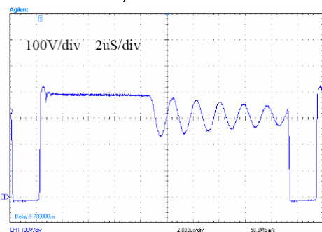
V in =220V, I o =0.5A
