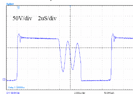
V in =110V, I o =0.5A
