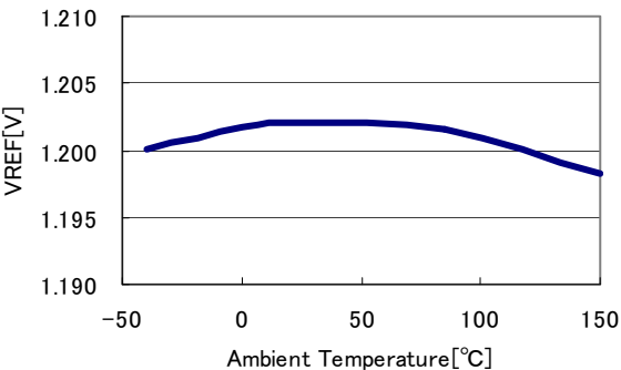
VREF vs Ambient Temperature
