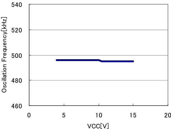
Oscillation Frequency vs VCC Voltage
