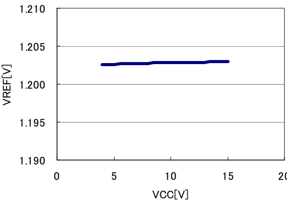
VREF vs VCC Voltage(Line Regulation)
