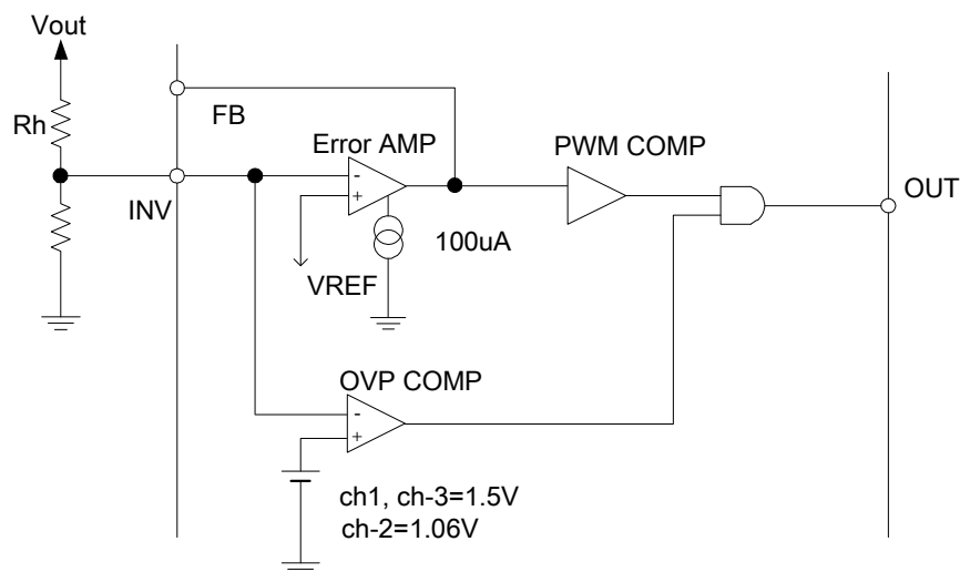
Figure 12. OVP Circuit
