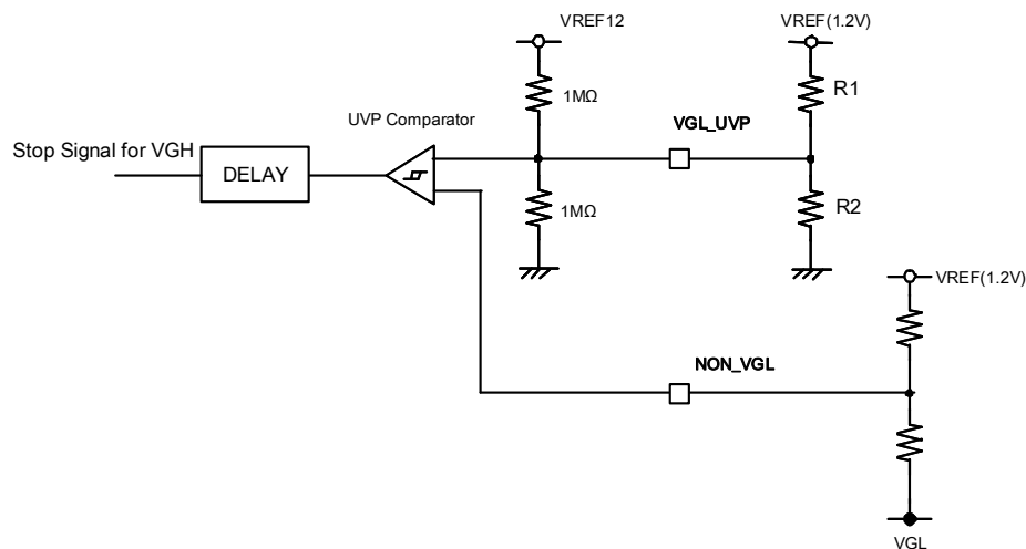
Figure 8. VGL_UVP Circuit
