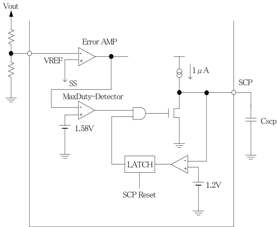
Figure 9. SCP Circuit
