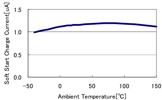
Soft Start Charge Current vs Ambient Temperature
