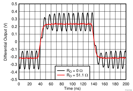
Figure 6-28. Step Response Into Capacitive Load
