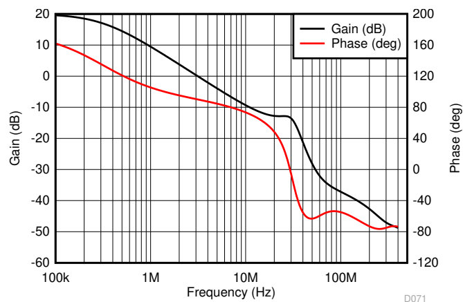
Figure 9-13. Gain and Phase Plot with a Differential Input Capacitor
