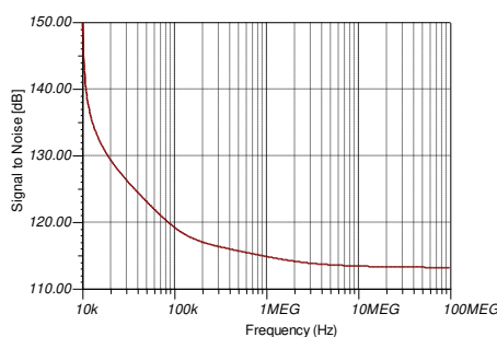
Figure 9-16. Signal-to-Noise Ratio Plot
