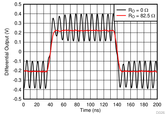
Figure 6-26. Step Response Into Capacitive Load
