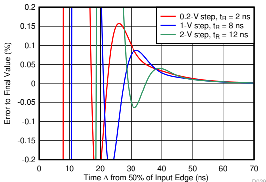
Figure 6-27. Small- and Large-Signal Step Response
