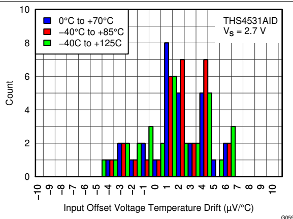
Figure 32. Input Offset Voltage Temp Drift Histogram
