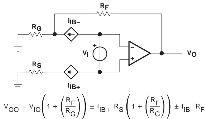
Figure 42. Output Offset Voltage Model
