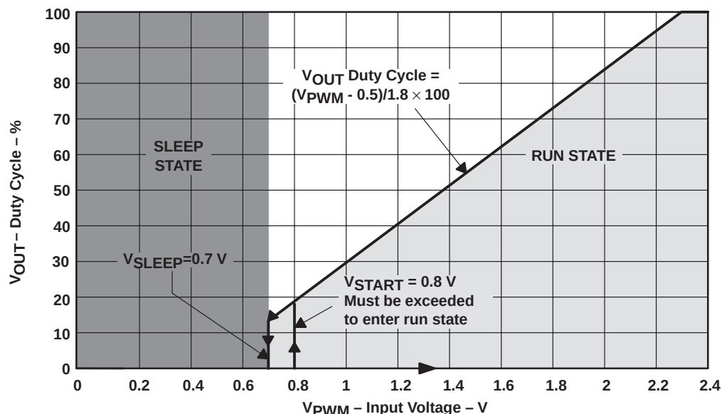
Figure 6. Relationship of V_{OUT} Duty Cycle, V_{START} , and V_{SLEEP} vs V_{PWM} Input Voltage
