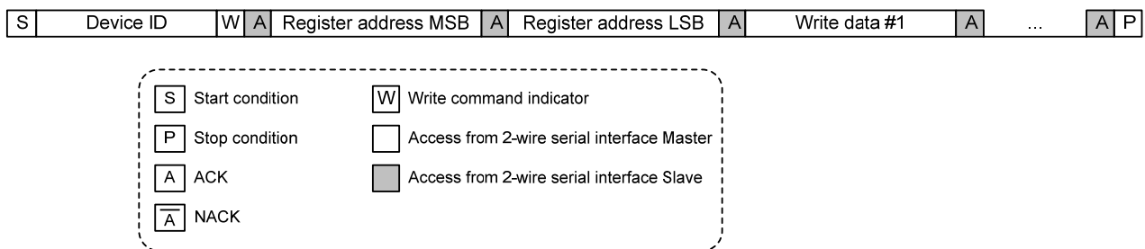
Figure 5. 2-wire serial I/F write to THCV242 local register protocol
