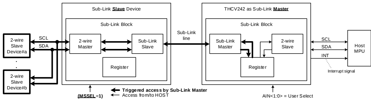
Figure 8. Host MPU to remote 2-wire slave devices via THCV242 access configuration
