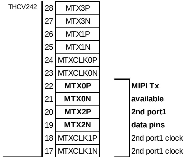
Figure 3. MIPI 2nd port available pins
