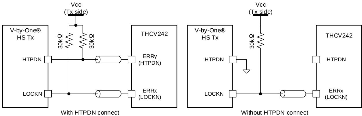
Figure 1. Physical wire connection for wired Hot-plug and Lock detect scheme
