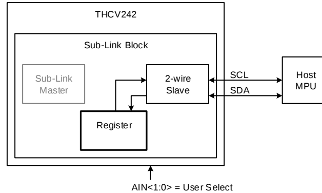
Figure 4. Host to THCV242 local register access configuration
