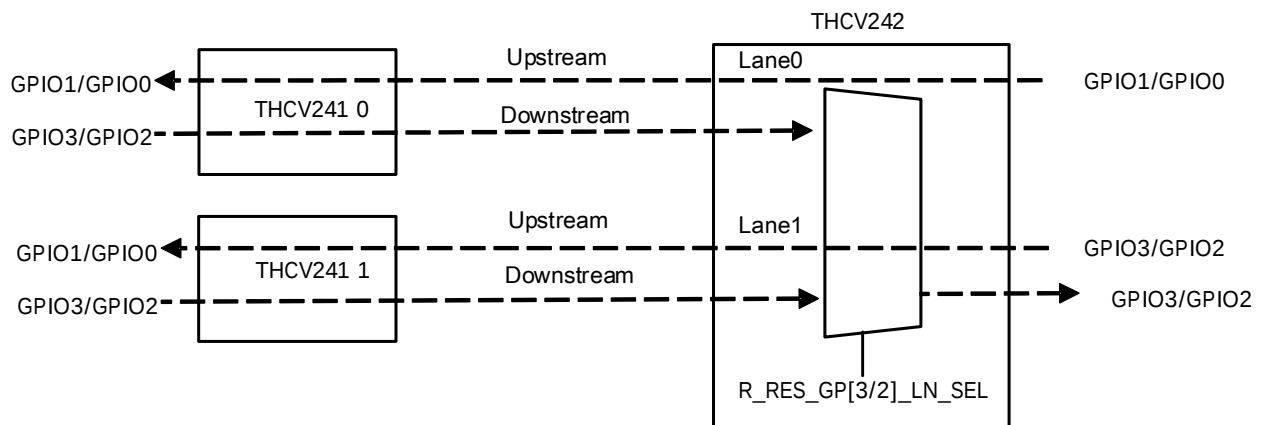
Figure 13. Through GPIO via Sub-Link transaction assignment with THCV241
