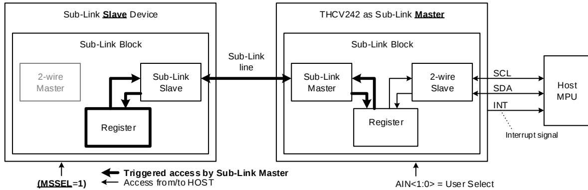
Figure 7. Host MPU to Sub-Link Slave Register via THCV242 access configuration
