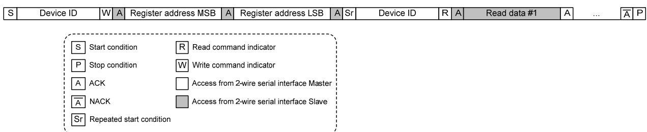
Figure 6. 2-wire serial I/F read to THCV242 local register protocol
