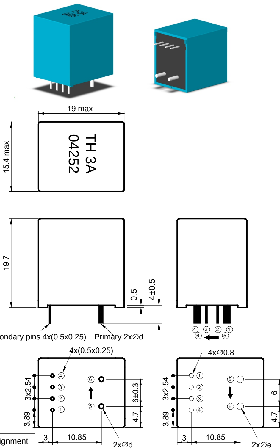
Bottom View
