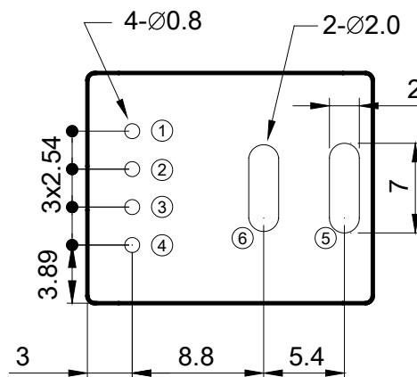
PCB mounting hole layout
