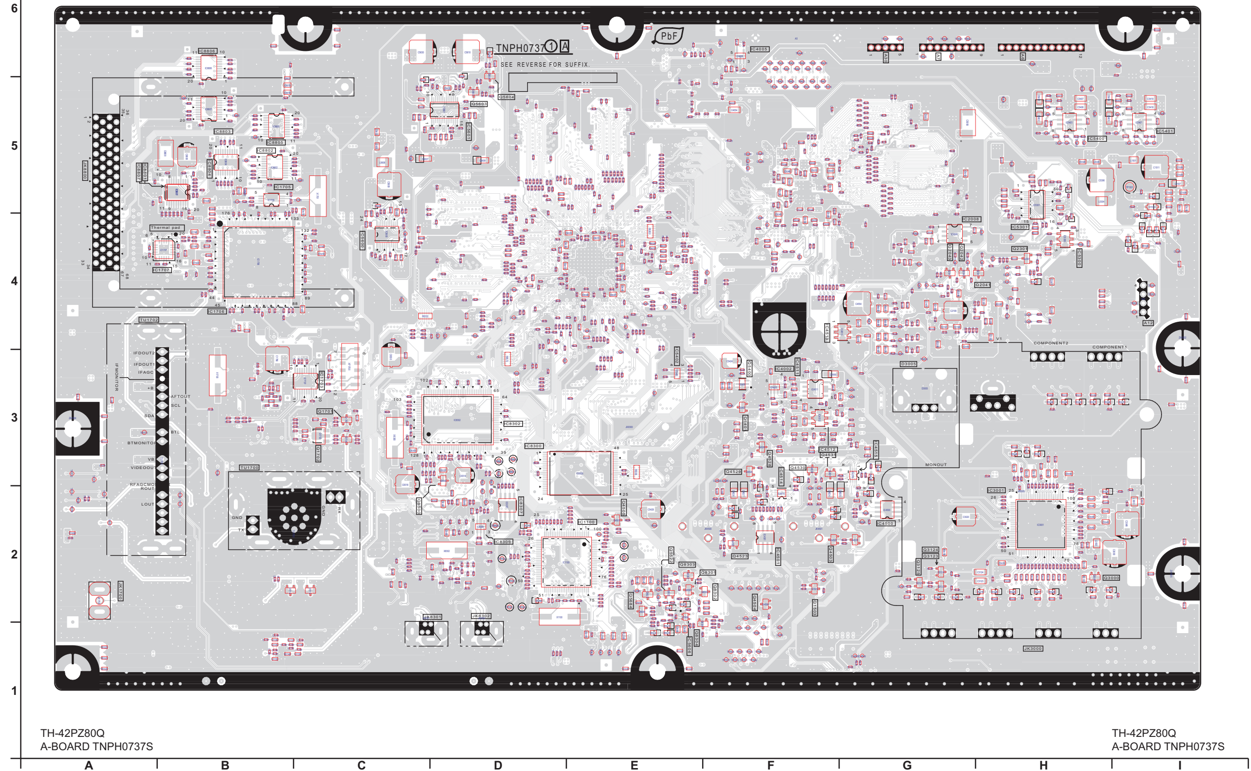
A-BOARD (FOIL SIDE) TNPH0737S
