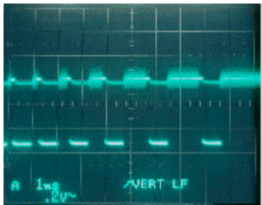
CN SC21, Pin 2 1ms / div, 0.2V CL
