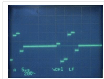
CN H2, Pin B15 5µs /div, 20mV Red Signal Input
