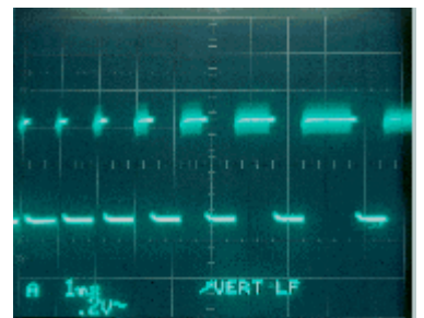
CN SC21, Pin 8 1ms / div, 0.2V CPL
