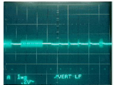
CN SC21, Pin 4 1ms / div, 0.2V SIU
