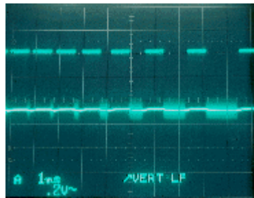
CN SC21, Pin 3 1ms / div, 0.2V CLK
