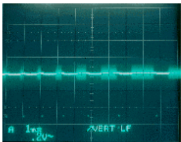
CN SC21, Pin 6 1ms / div, 0.2V SID
