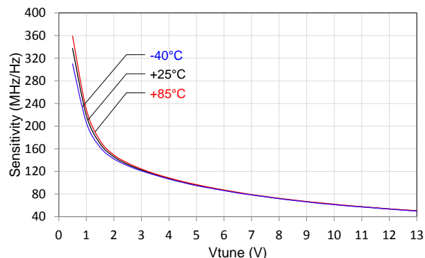
RFout/2 Sensitivity vs Tuning Voltage Vcc = 5V
