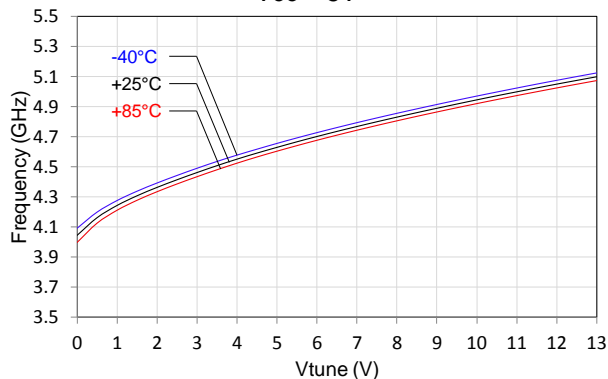
R Fout /2 Frequency vs Tuning Voltage V cc = 5V
