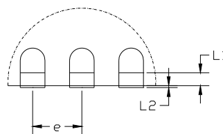
DETAIL B
