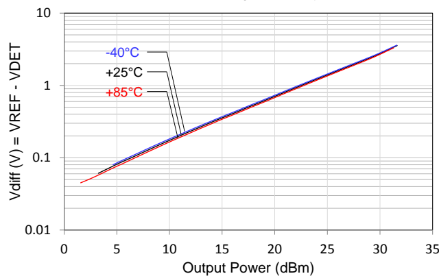
Power Detector vs. Pout vs. Temperature
