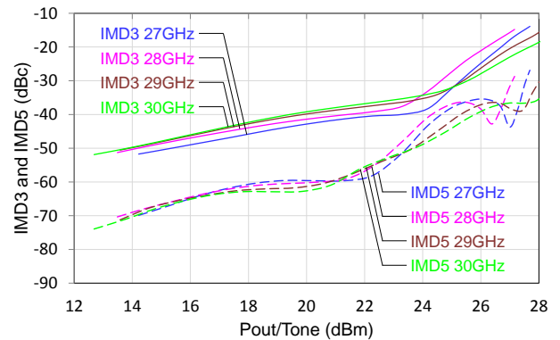
IMD3 and IMD5 vs. Pout/Tone vs. Frequency
