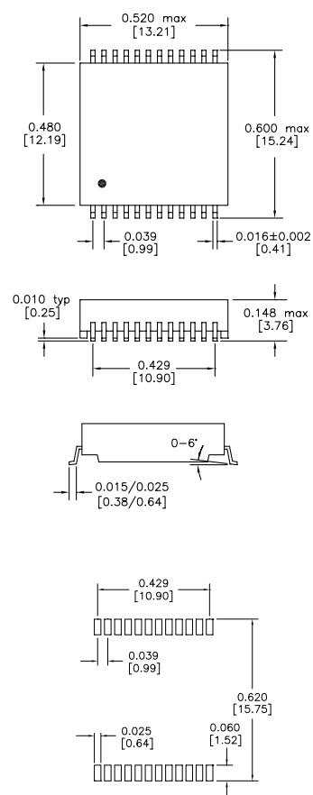
Recommended Solder Pad Layout
