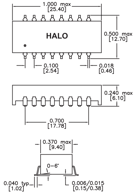
NL Package
