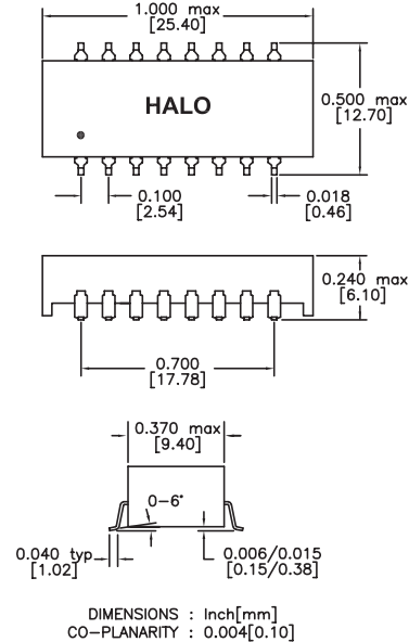
NL Package
