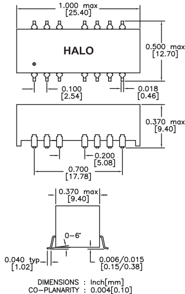
ND Package
