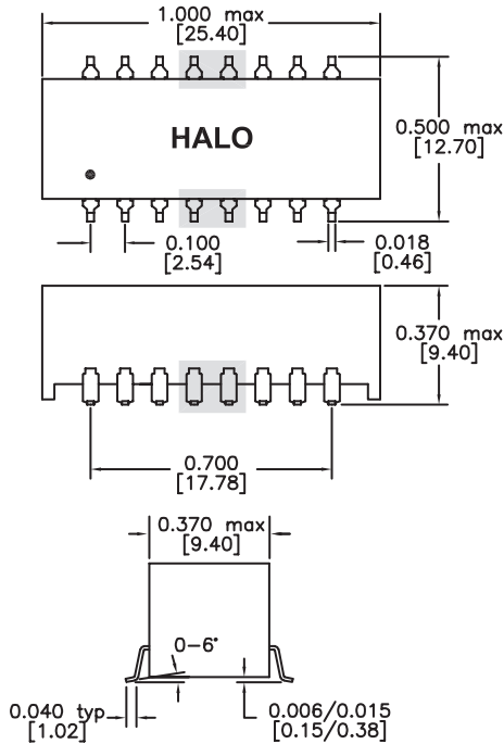
ND Package
