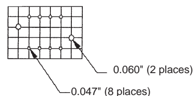
Hole arrangement View in mounting direction
