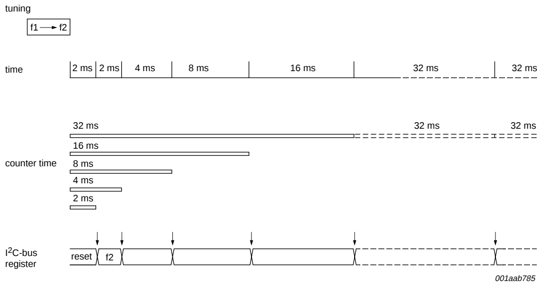
Fig 5. IF counter in FM mode after tuning
