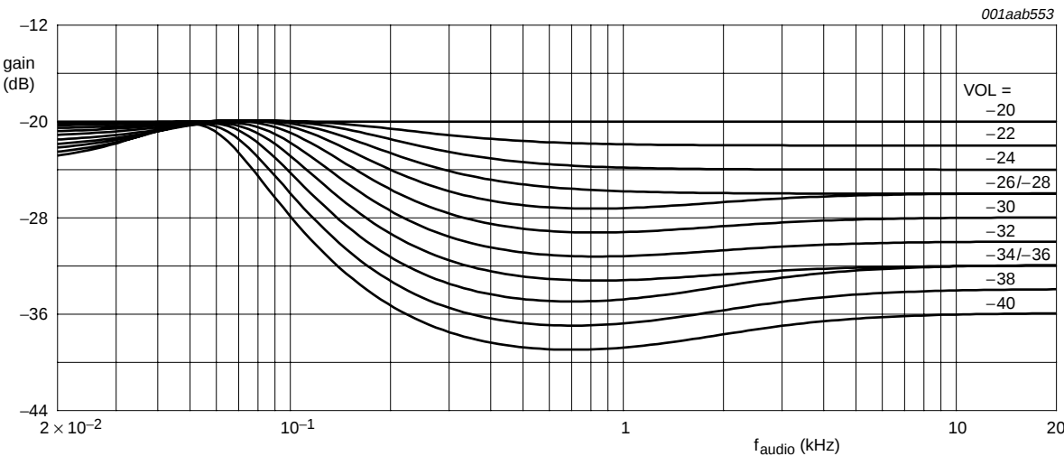
Fig 38. Loudness control characteristics; loudness start = −20 dB, bass frequency = 60 Hz, treble frequency = 10 kHz; bass gain = 0 dB, treble gain = 0 dB
