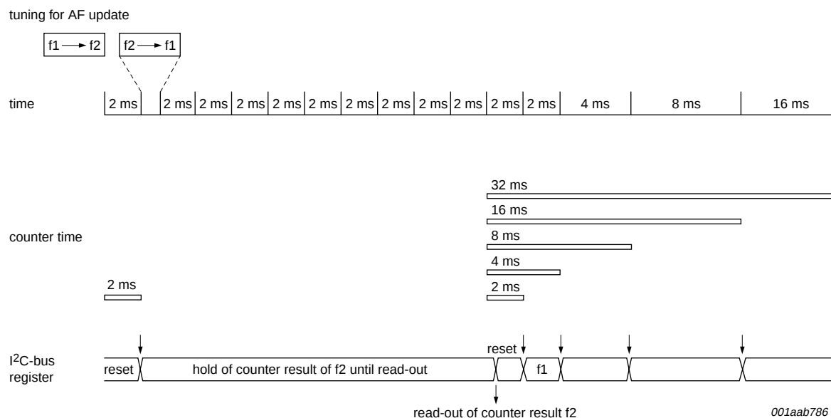
Fig 6. IF counter in FM mode during and after AF update
