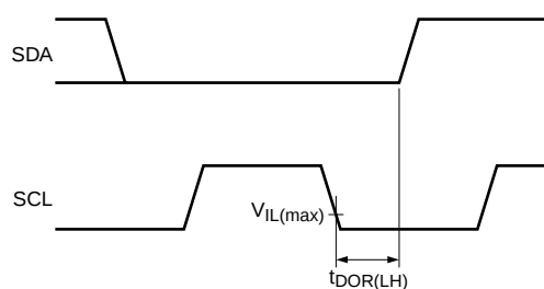
Fig 42. Data output reaction time of the IC
