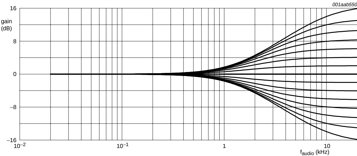
Fig 37. Treble amplitude control characteristics; treble frequency (TRF) = 10 kHz
