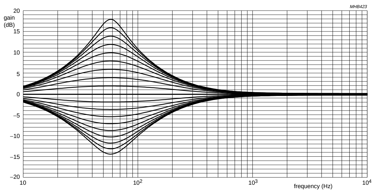
Fig.18 Bass curve with 2 \times 220 nF and R = 3.3 k \Omega external, BSYB = 1 and BSYC = 1.
