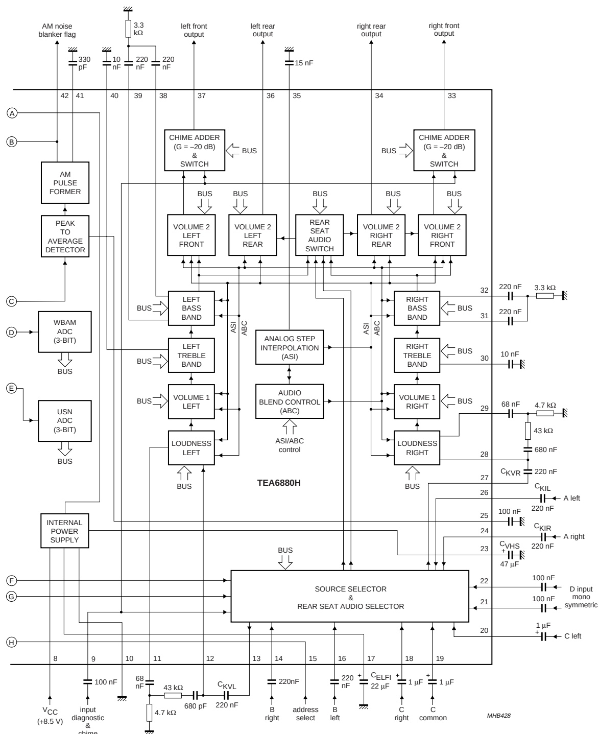
Fig.2 Block diagram (continued from Fig.1).
