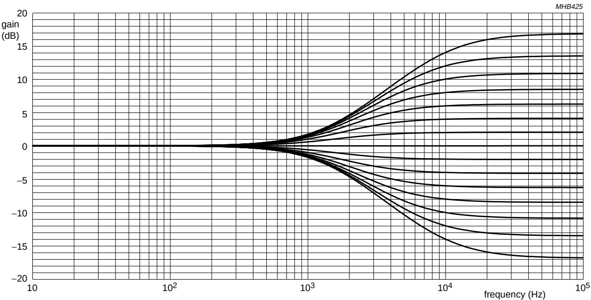
Fig.20 Treble control characteristic.
