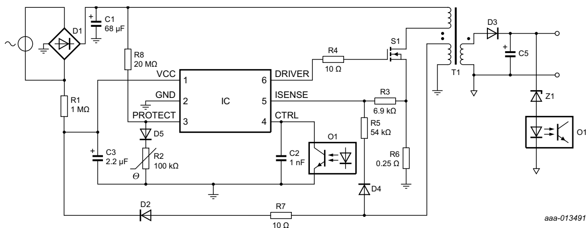
Fig 14. TEA1832LTS application diagram
