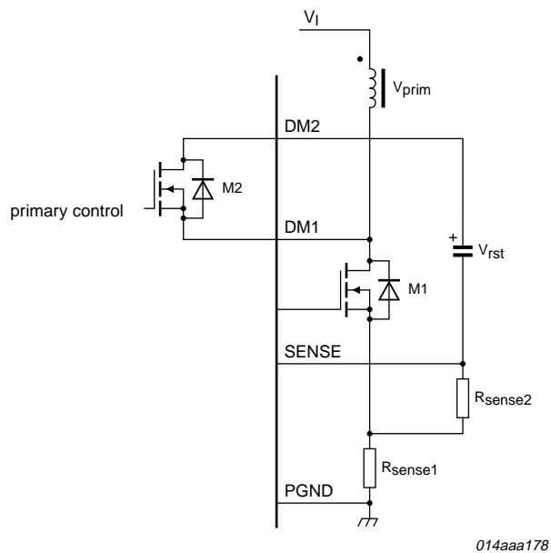
Fig 10. Current sense circuit
