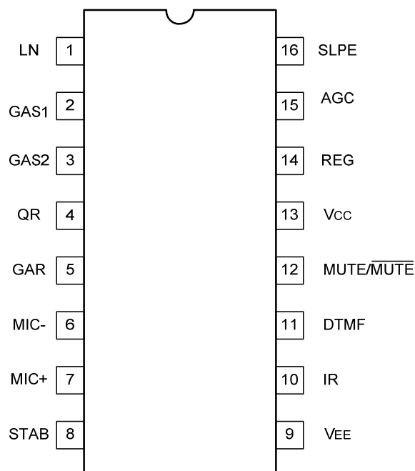
Fig. 1 Pin Configurations
