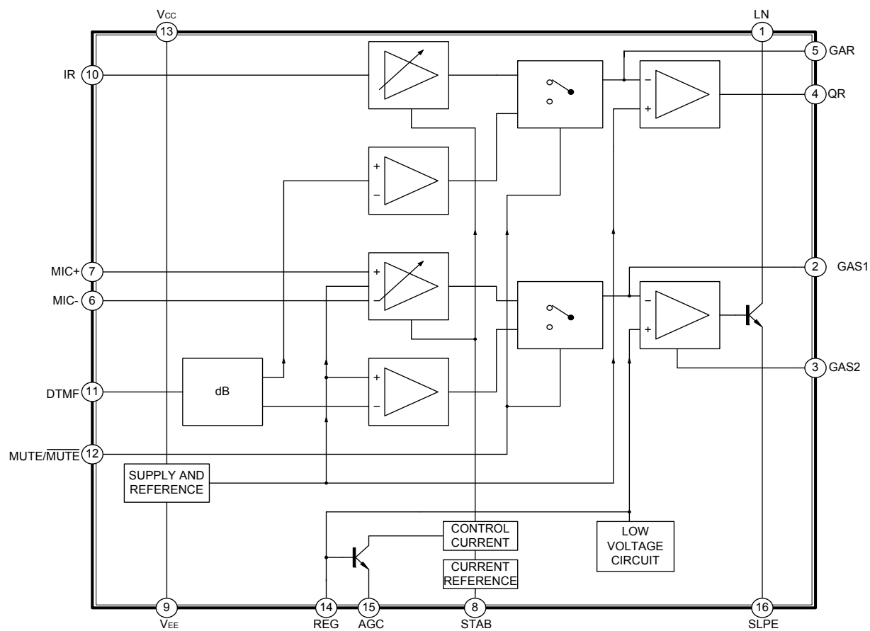
Fig. 2 Block Diagram
