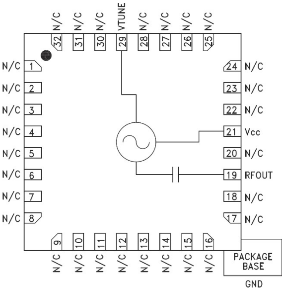
Figure 1: Package Pinout
