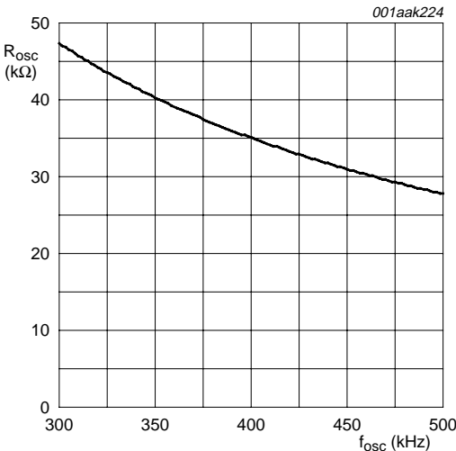
Fig 4. Clock frequency as a function of R OSC
