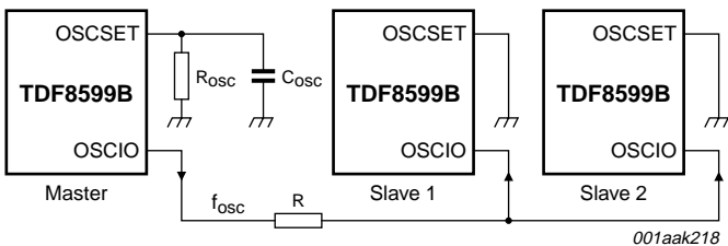
Fig 5. Master and slave configuration
