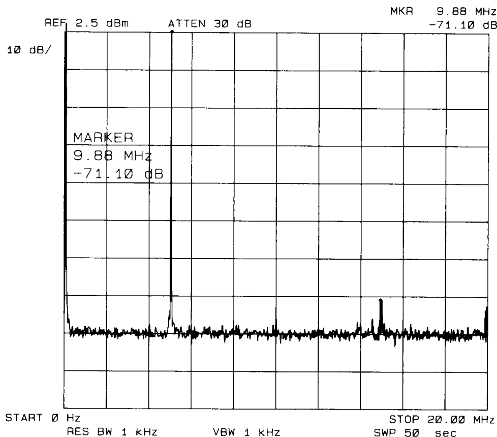
Figure 8. Typical Output Spectrum, 40Mps, 5MHz F OUT
