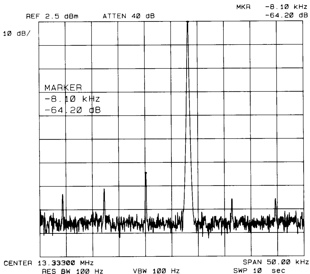
Figure 7. Typical Output Spectrum, 40MSPS, 13.336MHz F OUT
