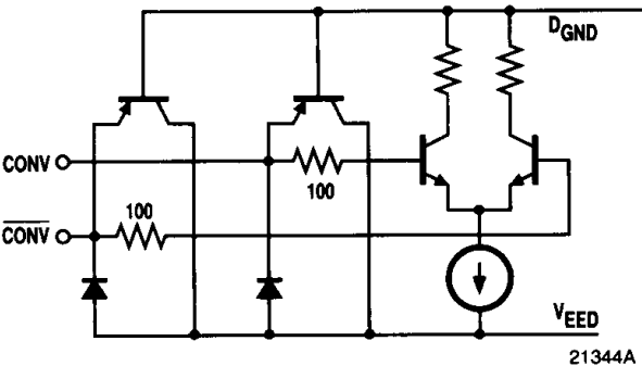
Figure 2b. Equivalent Input Circuit (CONV and \overline{CONV} )
