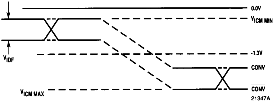
Figure 5. CONV and \overline{CONV} Switching Levels
