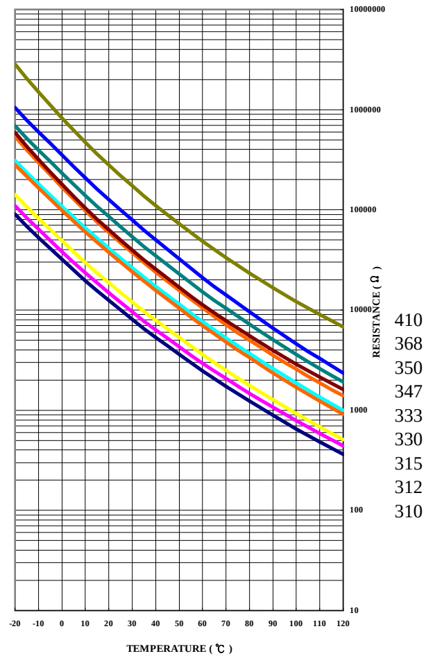
Typical R-T Curves of TDC 3mm Series
