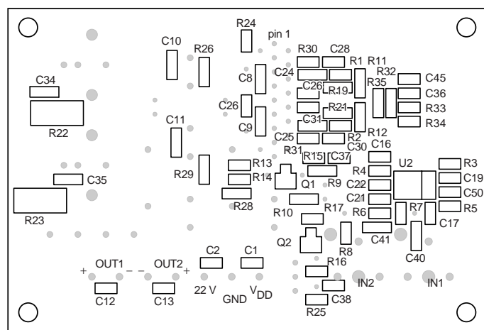
Bottom silk
