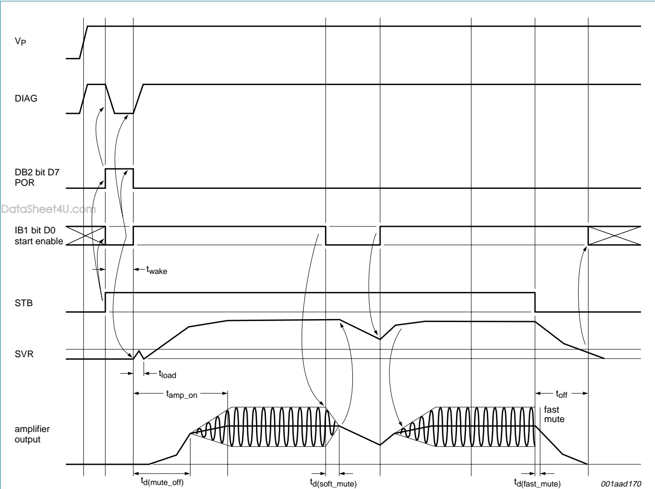
Fig 6. Start-up and shut-down timing with low audible pop and DC load activated
