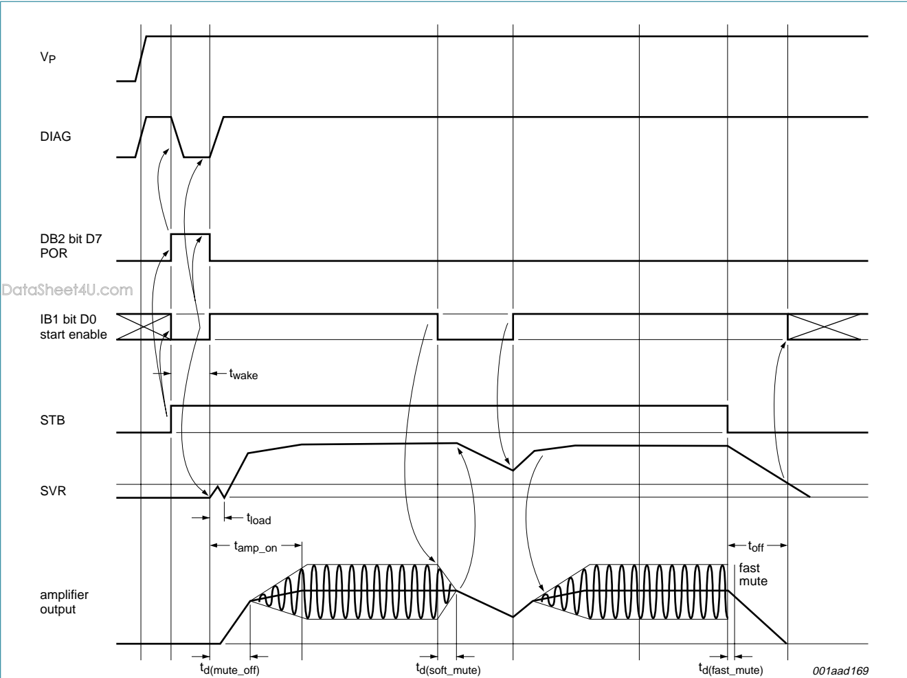
Fig 5. Start-up and shut-down timing with DC load active in I 2 C-bus mode
