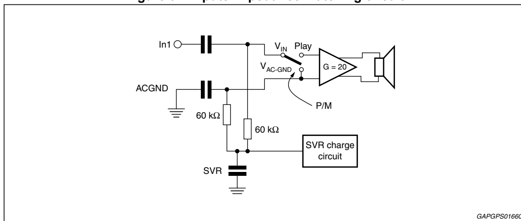
Figure 37. Inputs impedance matching circuit
