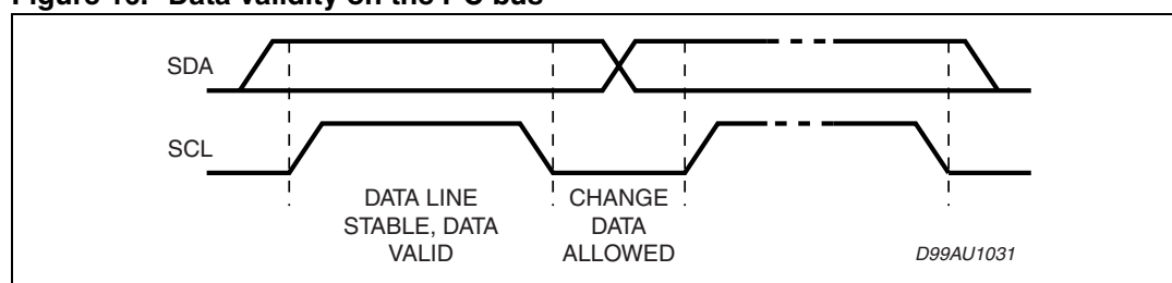
Figure 17. Timing diagram on the I 2 C bus
