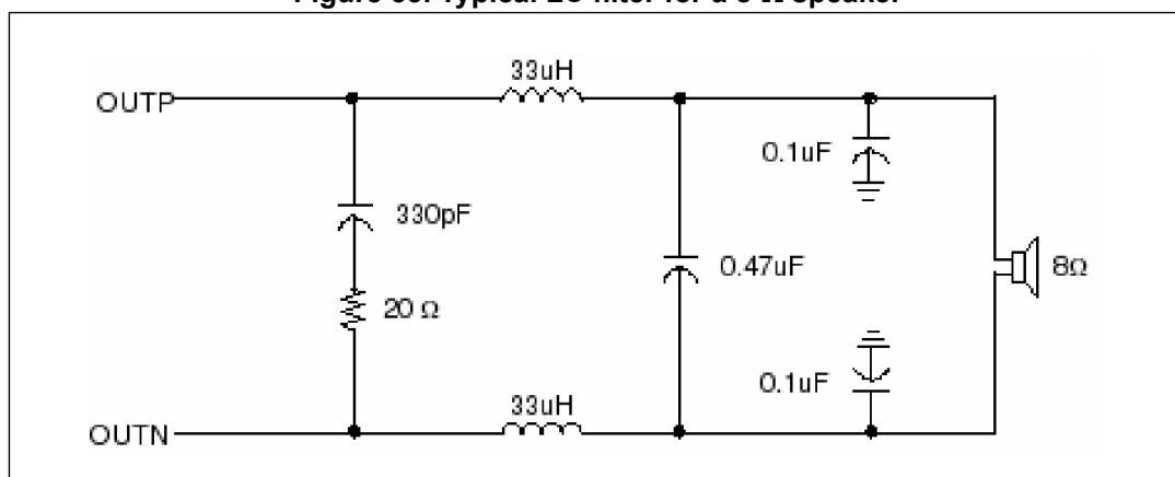
Figure 33. Typical LC filter for a 8-Ω speaker
