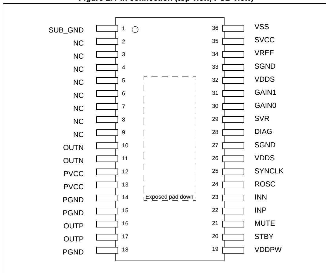
Figure 2. Pin connection (top view, PCB view)
