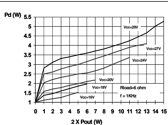
Figure 8. dissipated power vs output power
