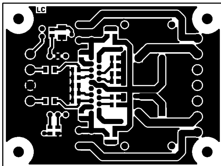
Figure 15. PCB copper top (top view)
