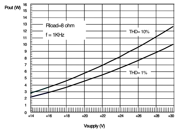
Figure 4. output power vs supply voltage (single)
