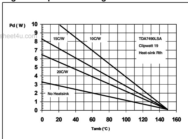
Figure 11. power derating curve
