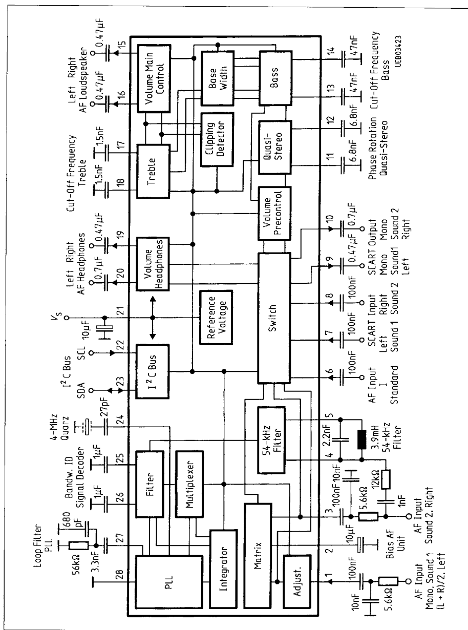
Application Circuit 3
