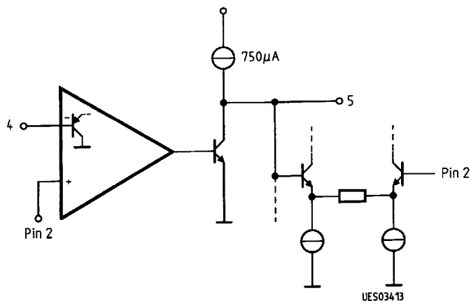
54-kHz Filter (Pin 4/5)
