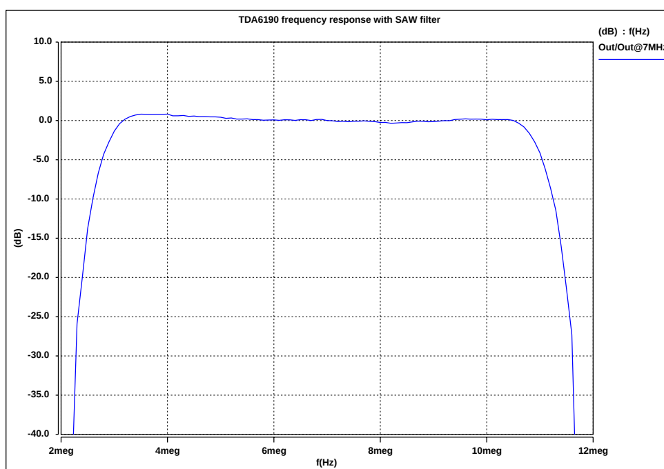
TDA6190_FrequencyResponse.pdf
