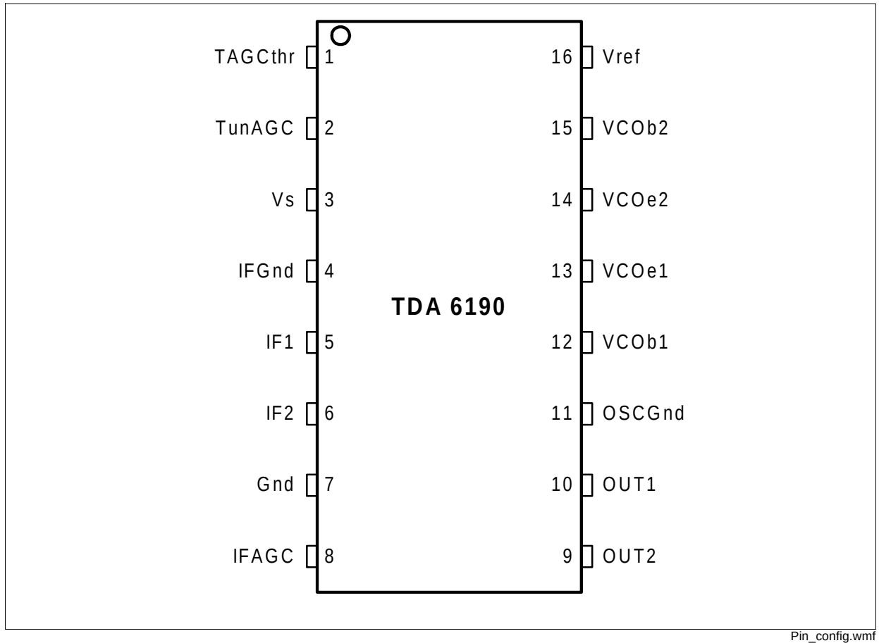
Figure 2-1 Pin Configuration
