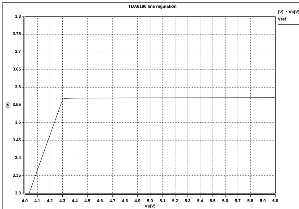
TDA6190_LineRegulation.pdf
