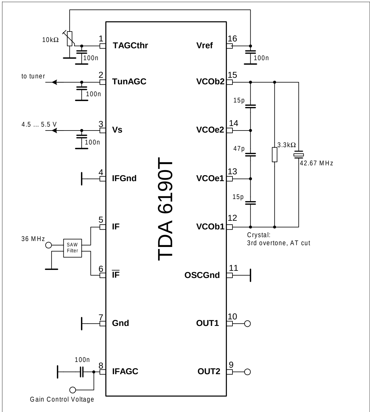
Figure 3-3 Application Circuit 2
