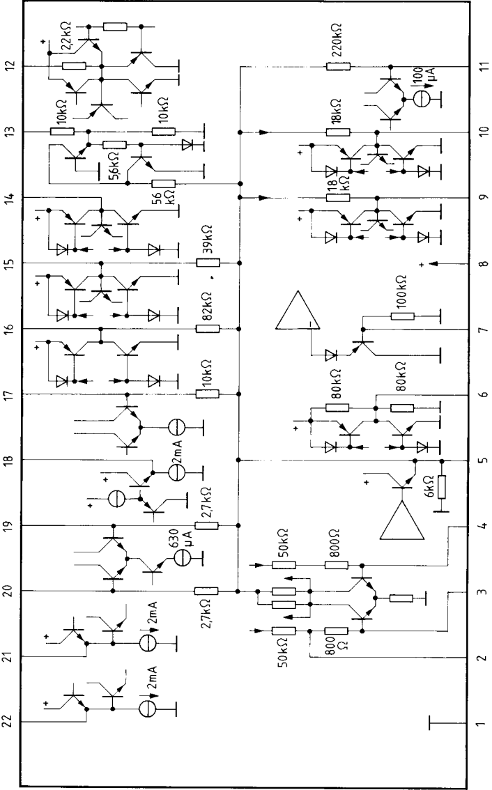
Internal pin Diagram
