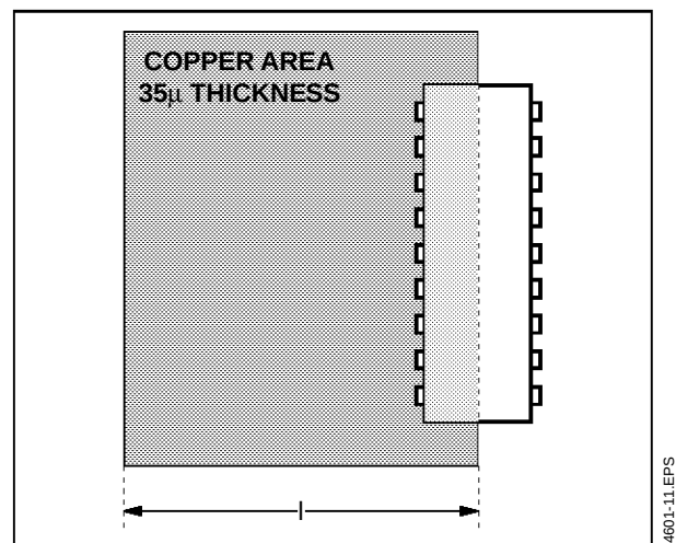
Figure 7 : Example of a PC Heatsink ( 35^\circ\text{C/W} )
