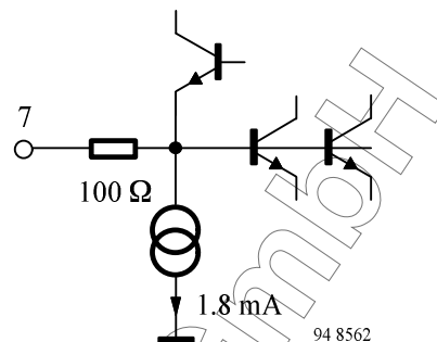
Figure 9. Audio output – SCART (Pin 7)
