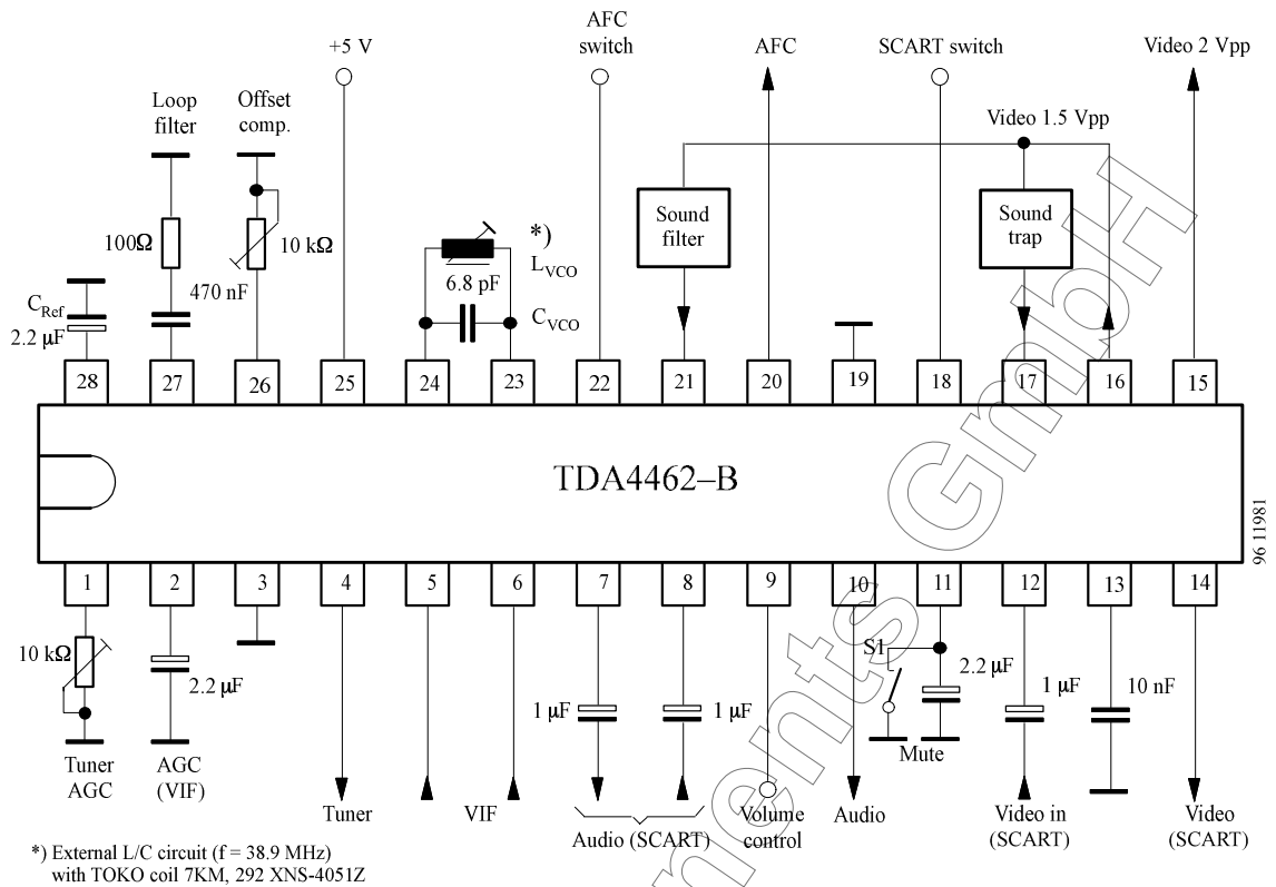
Figure 3. Test circuit
