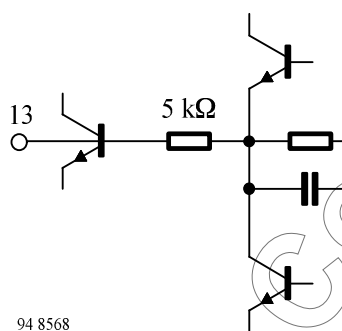
Figure 15. De-emphasis (Pin 13)
