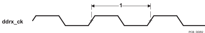
Figure 8-37. DDR2 Memory Controller Clock Timing
