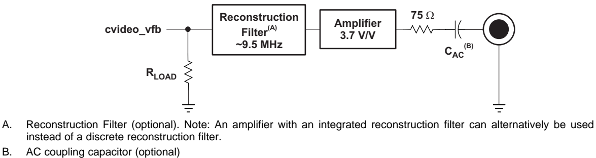
Figure 8-73. TV Output (TVOUT Bypass Mode)
