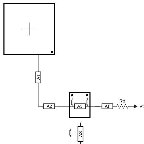
SPRS91v_PCB_DDR3_11
