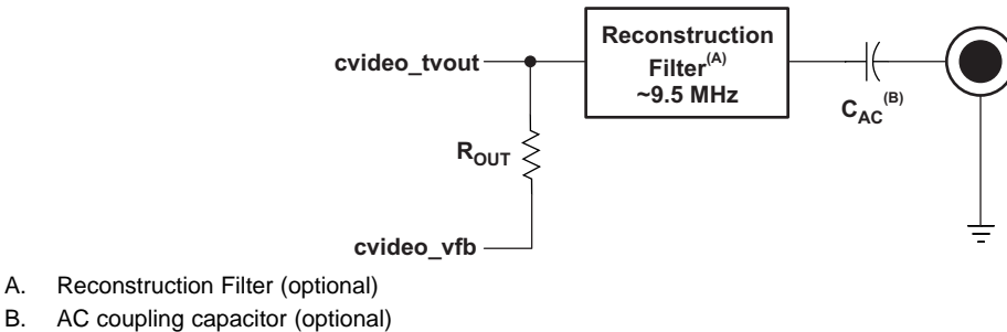
Figure 8-72. TV Output (Normal Mode)
