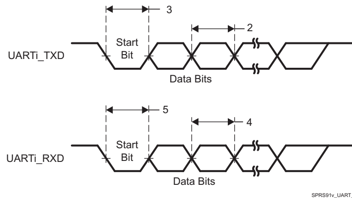
Figure 7-25. UART Timing
