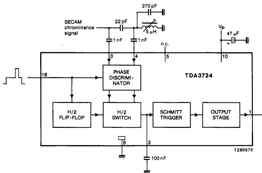
Fig. 1 Block diagram.
