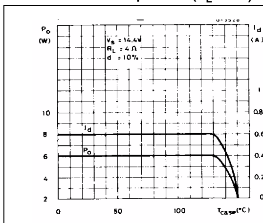
Figure 24. Output power and drain current vs. case temperature ( R_L = 4 \Omega )
