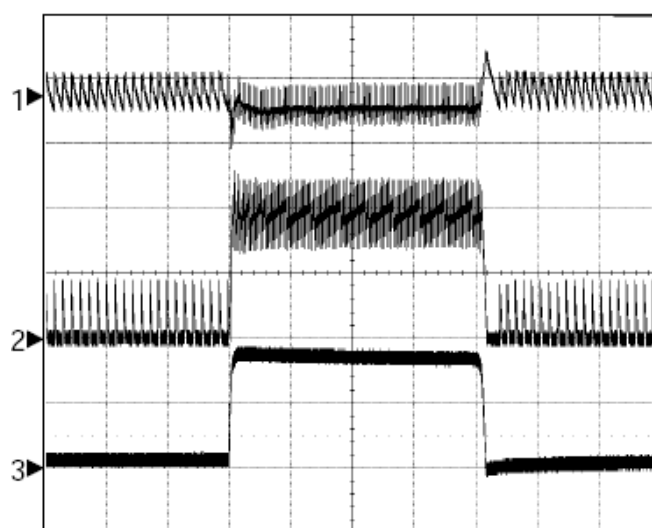
V_{OUT}=1.1V , Load Transient 1A->18A->1A
