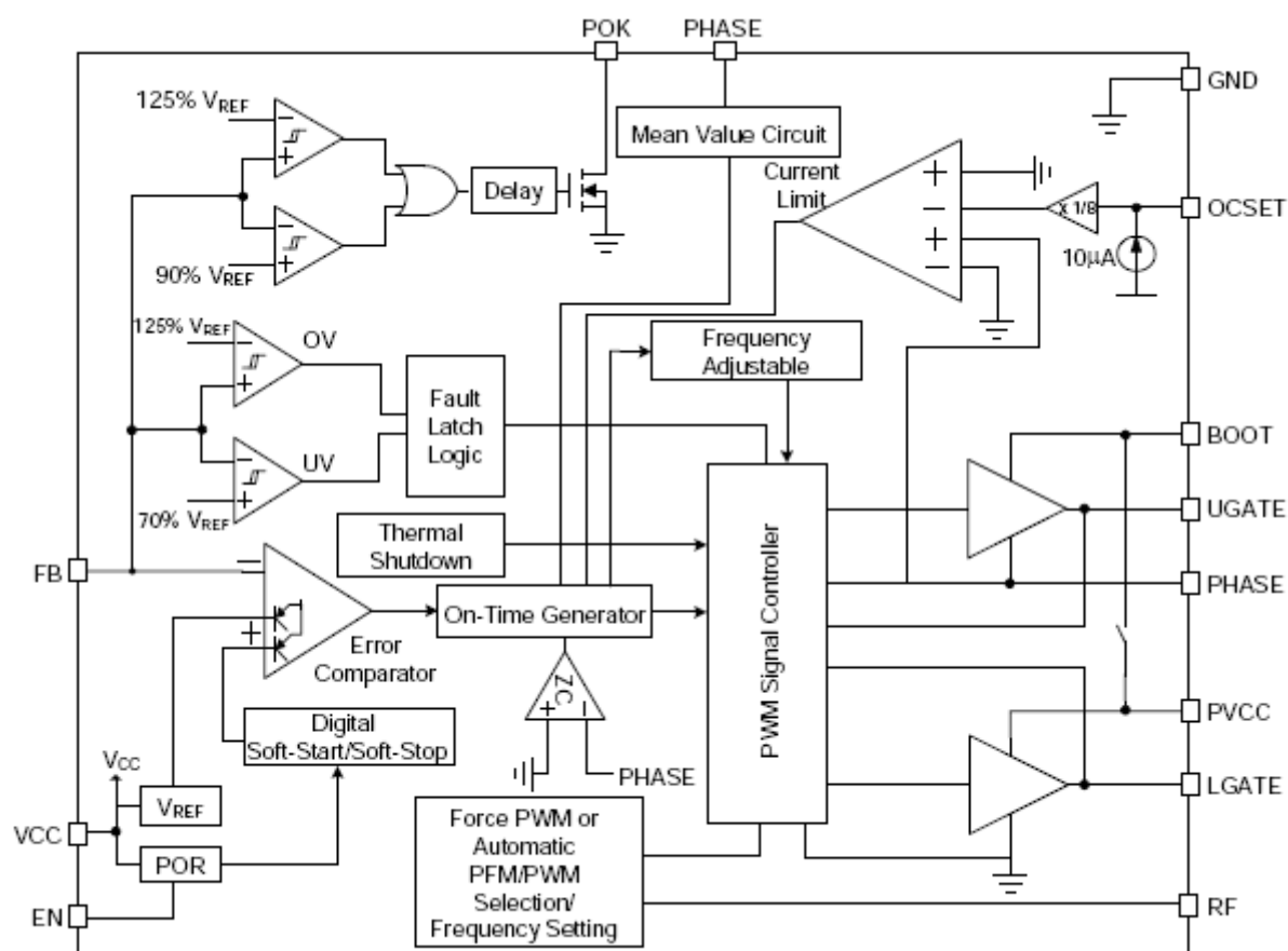
Functional Block Diagram of TD1729
