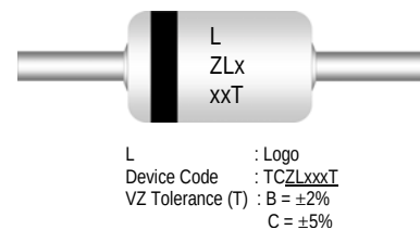
DEVICE MARKING DIAGRAM
