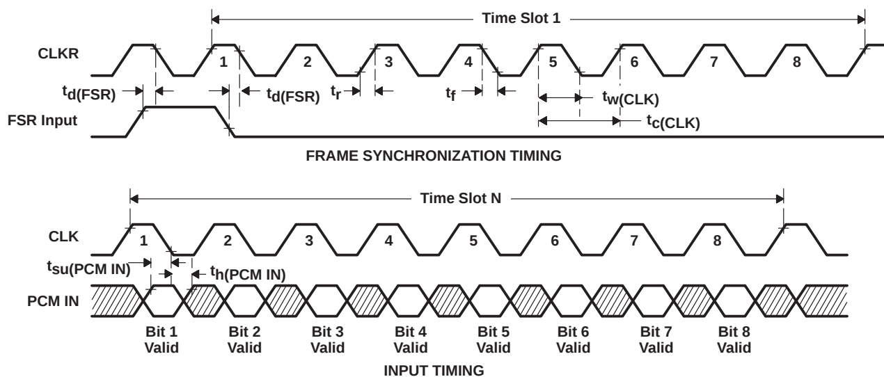
Figure 3. Transmit Timing (Fixed-Data Rate)
