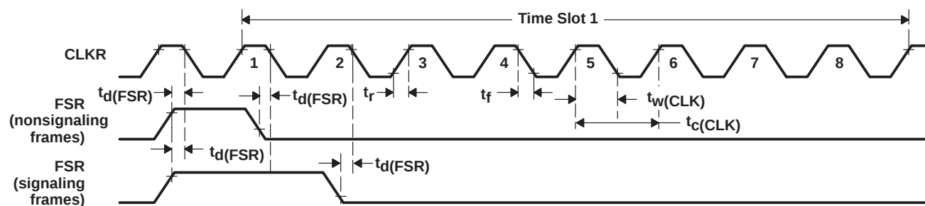
FRAME SYNCHRONIZATION TIMING
