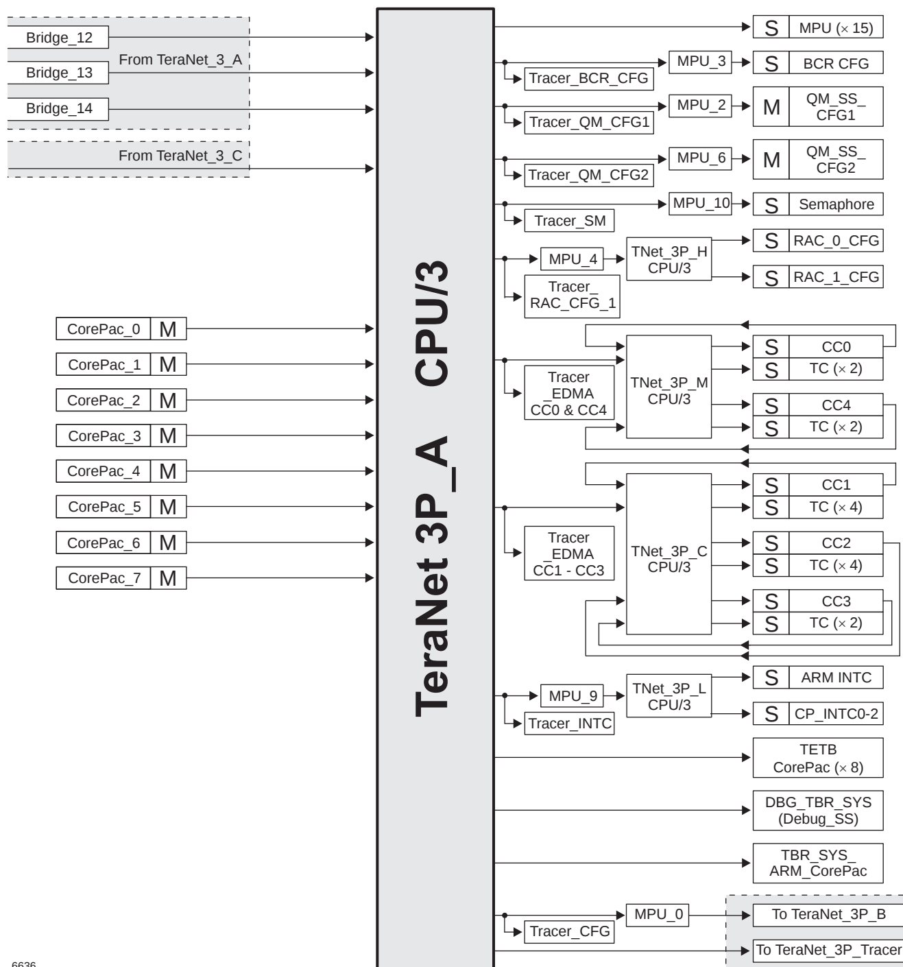
Figure 7-5 TeraNet 3P_A
