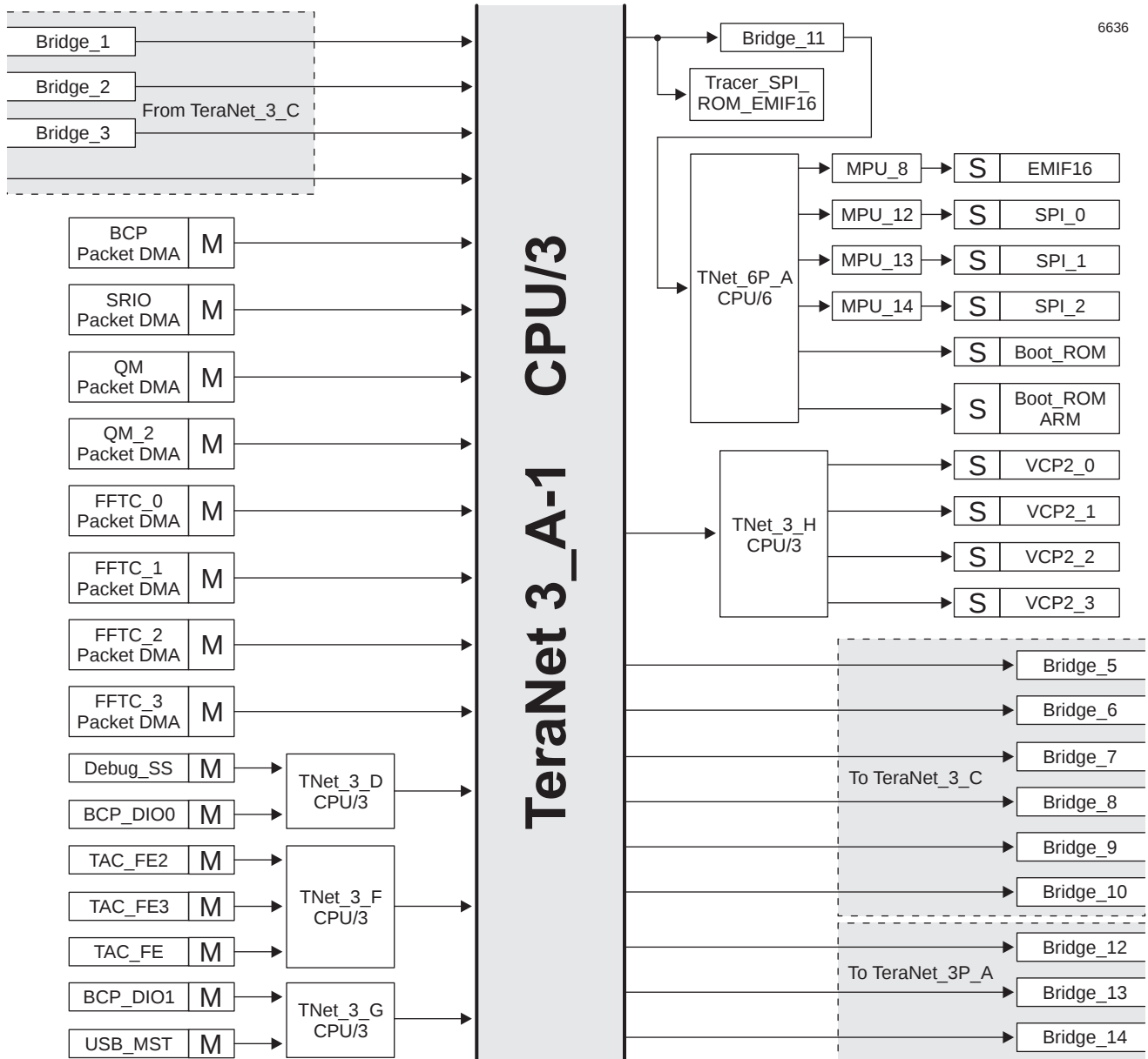
Figure 7-1 TeraNet 3_A-1
