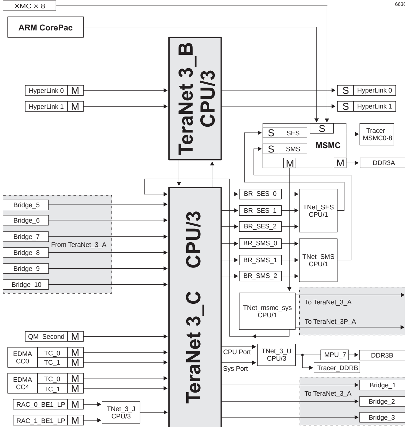
Figure 7-3 TeraNet 3_C
