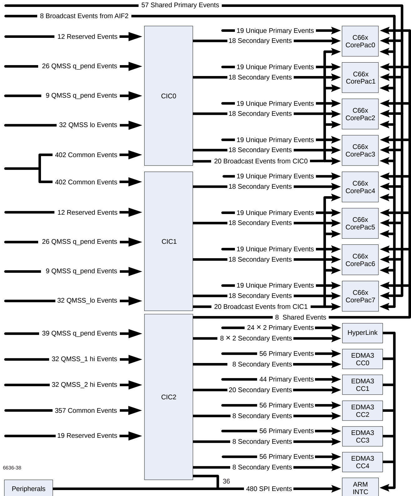
Figure 6-5 Interrupt Topology
