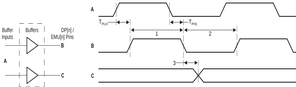
Figure 10-62 Trace Timing
