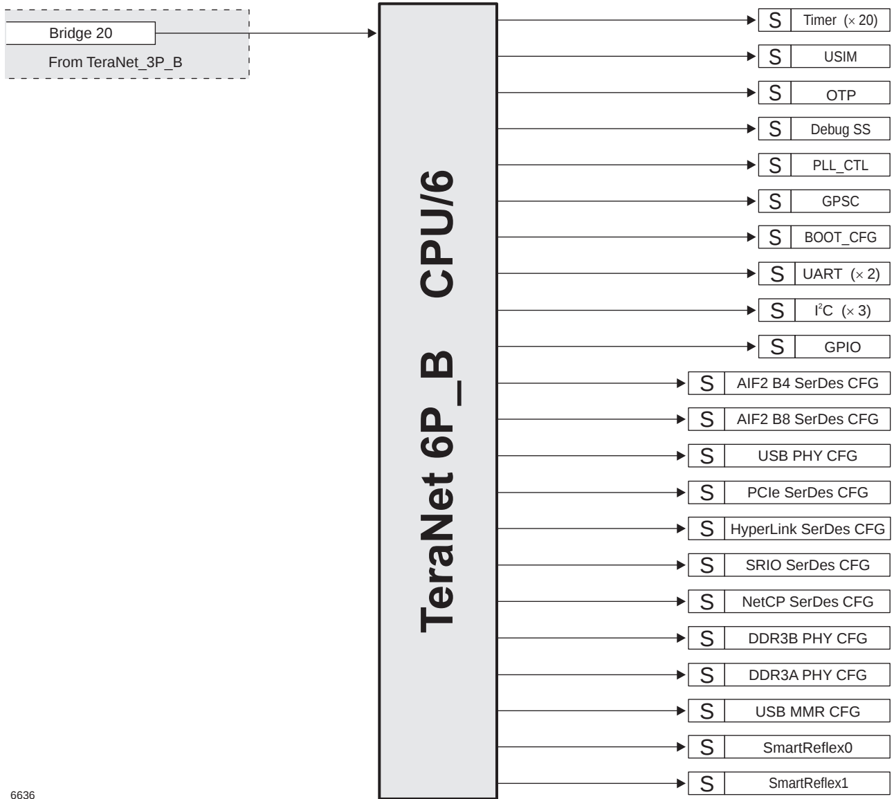
Figure 7-7 TeraNet 6P_B
