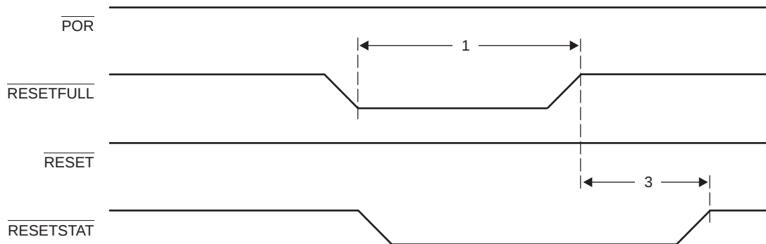
Figure 10-4 RESETFULL Reset Timing
