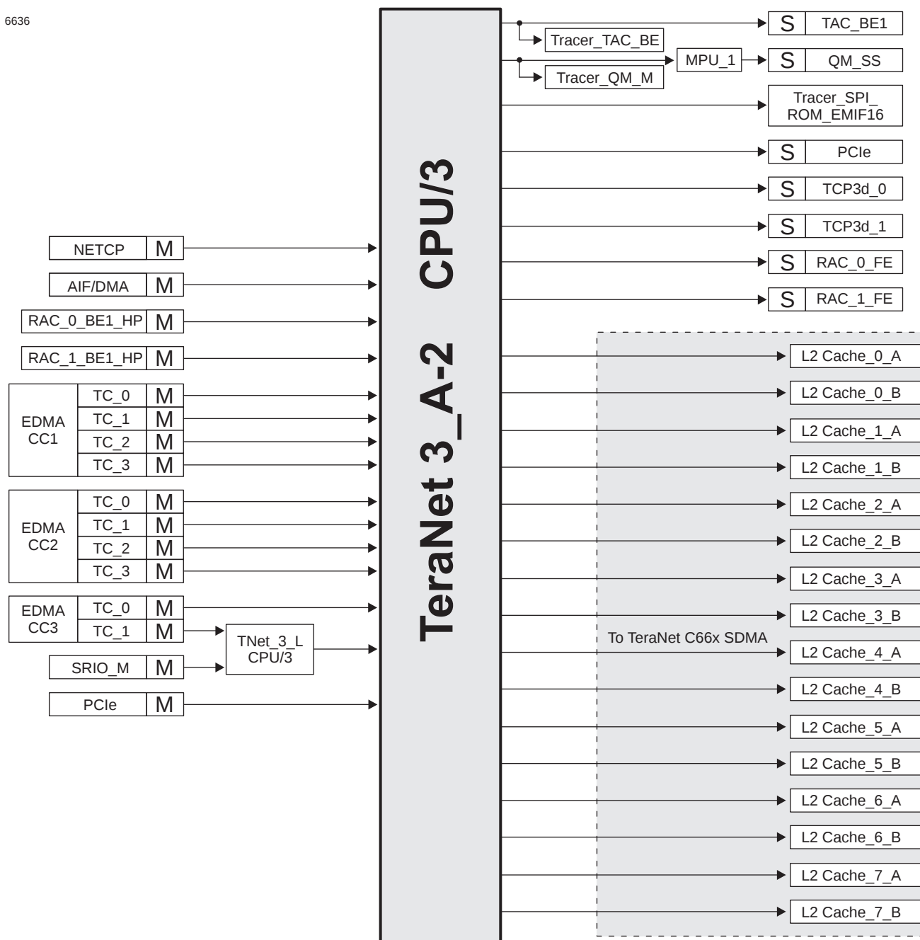
Figure 7-2 TeraNet 3_A-2
