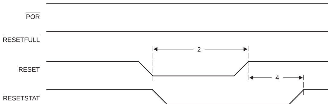
Figure 10-5 Soft/Hard Reset Timing
