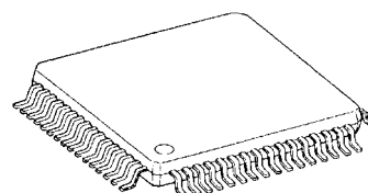
LQFP64-P-1010-0.50
